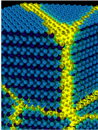
Figure 1. Artist's depiction of the collective excitations of an exciton condensate. These excitations can be thought of as propagating domain walls (yellow) in an otherwise ordered solid exciton background (blue). Image courtesy of Peter Abbamonte, University of Illinois Department of Physics and Frederick Seitz Materials Research Laboratory.
